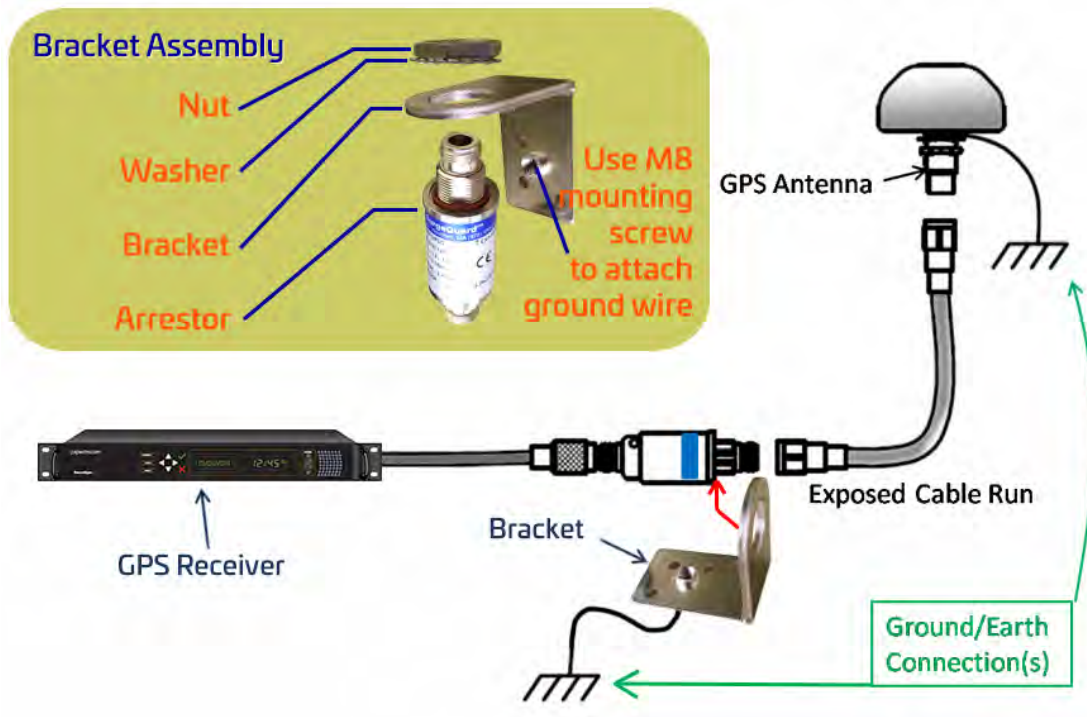
Figure 1-2: Model 8226 with optional mounting bracket
