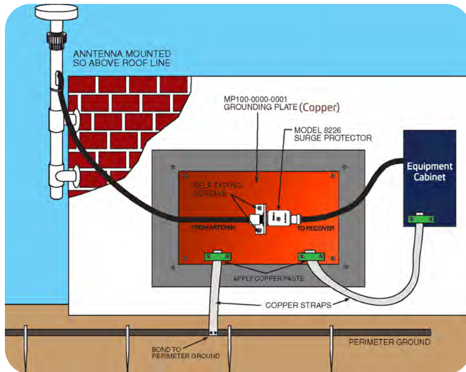
Figure 1-3: Grounding kit panel installation
