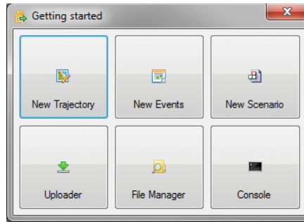
Figure 1: Start Menu
