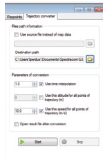
Figure 4: Trajectory Converter
