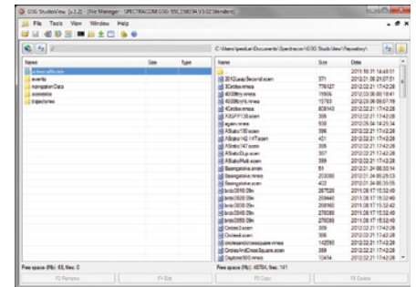
Figure 7: File Manager
