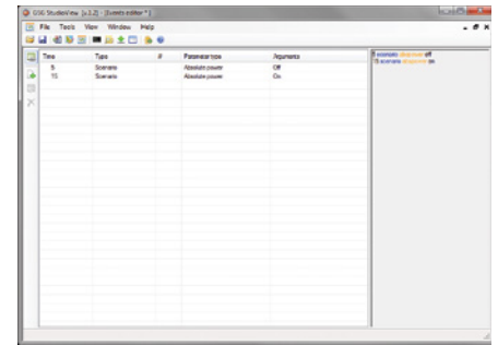
Figure 5: Event Parameters
