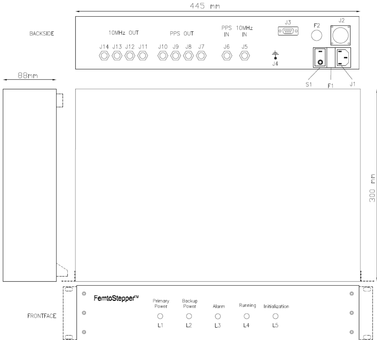
Figure 2- Mechanical Outline
