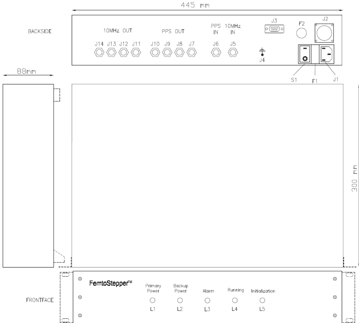
Figure 2- Mechanical Outline
