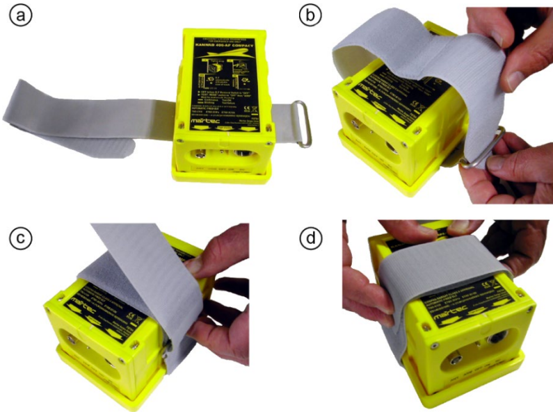
Figure 3: Securing the ELT
