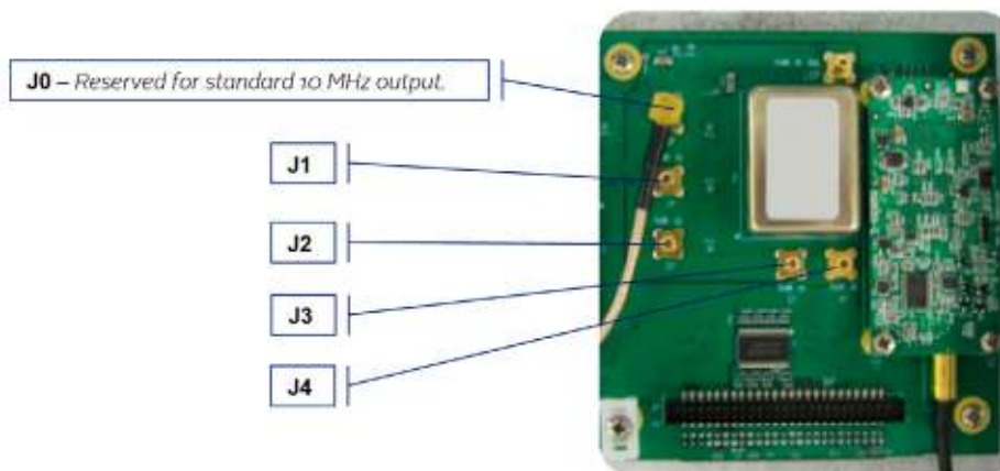
Figure 8: J Connectors
