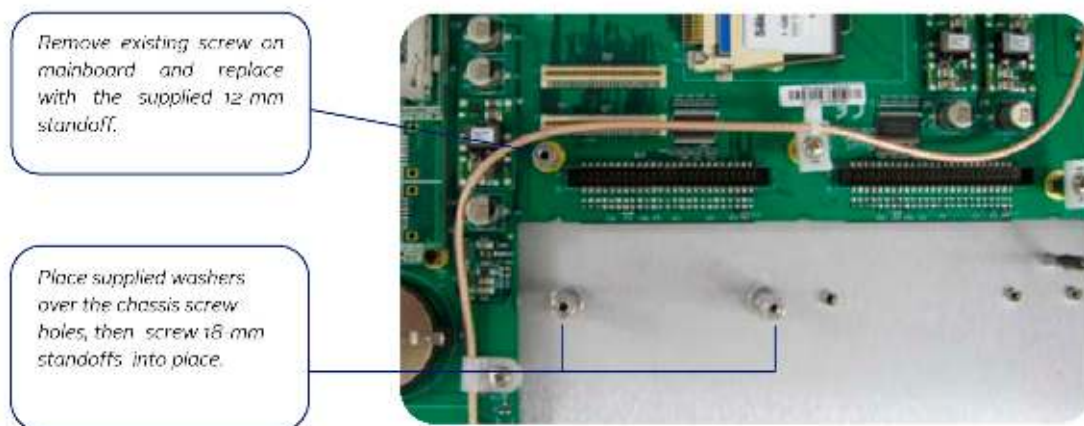
Figure 10: Gigabit Ethernet option card installation
