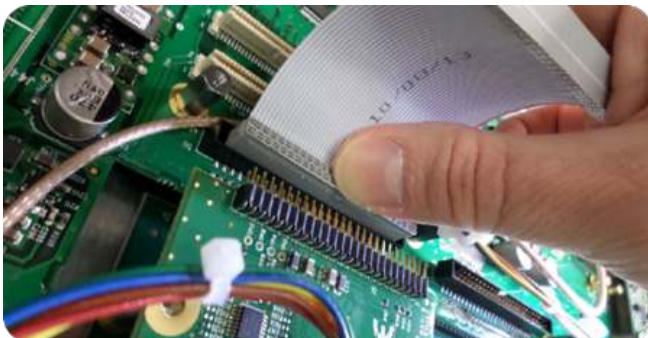
Figure 5: Ribbon cable installation
