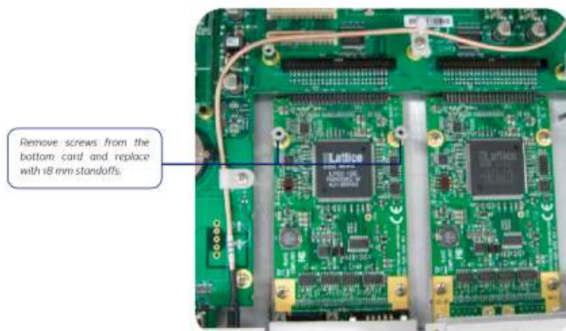
Figure 6: Bottom card with standoffs installed
