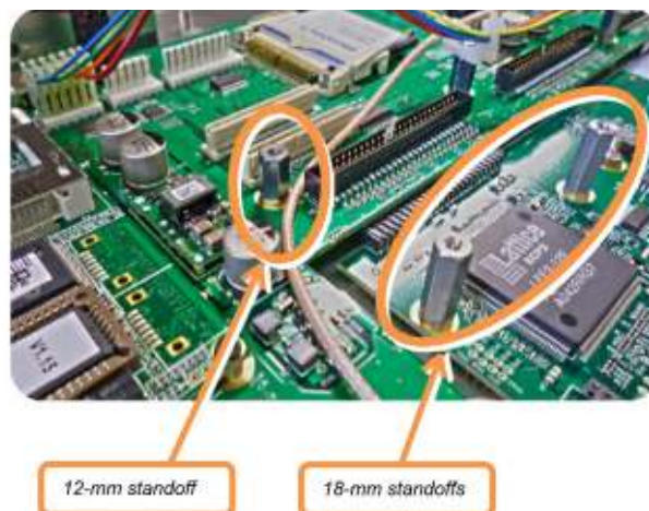
Figure 11: Gigabit Ethernet option card installation
