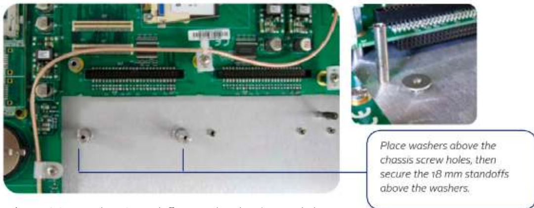
Figures 3 & 4: Washers & standoffs secured to chassis screw holes
